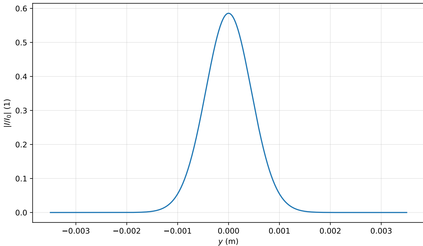
Intensity profile I(x=0, y, z=1.831)/I_0 , P_{in}=0.1P_{cr} , artificial time
